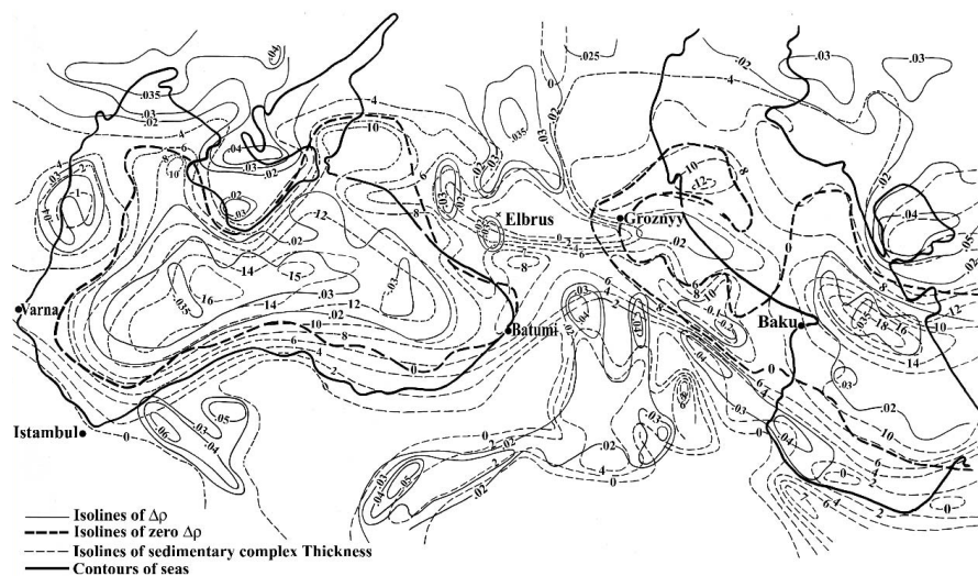
Fig. 5. The map of sedimentary complex thickness ( H ) and thermodense anomalies ( \Delta\rho ).
