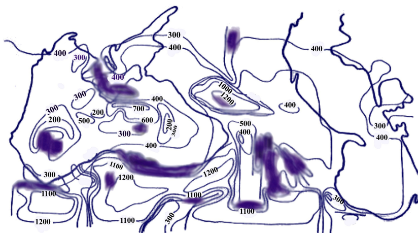
Fig. 4. Vertical thermodisplacements of the Caucasus and the Black and the Caspian Seas water areas.
